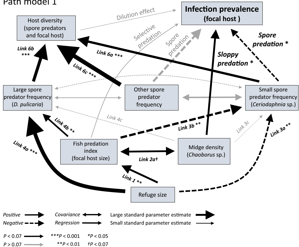
FIG. 6. Path model 1 disentangles drivers of infection prevalence in a focal host ( Daphnia dentifera ). Ecological links among habitat, predators, and host diversity (Links 1–4 and 6, Table 2; Figs. 3 and 5) synthesize three modes of predation (Table 1; Fig. 2). From the bottom, moving up: (1) Small refuges led to intense selective fish predation. (2a) Intense fish predation correlated with low density of sloppy midge predators ( Chaoborus ). (3a) Small refuges and (3b) intense fish predation increased frequency of small spore predators ( Ceriodaphnia ) in the host community. (4a) Large refuges and (4b) less-intense fish predation increased frequency of large spore predators ( D. pulicaria ). (6a–c) Frequencies of all spore predators increased host diversity. Disease drivers: Sloppy midge predators and small spore predators ( Ceriodaphnia ) had large, significant, and direct effects on infection prevalence. Selective fish predation did not directly drive infection prevalence, but indirectly mediated density of sloppy midge predators and frequency of small spore predators. Other spore predators reduced disease, but not significantly. The dilution effect pattern was not significant, once accounting for the direct effects of small spore predators and other spore predators. Model fit statistics: Satorra-Bentler chi square P = 0.903 ; comparative fit index (CFI) = 1.000; Tucker-Lewis index (TLI) = 1.152; root mean square error of approximation (RMSEA) = 0.000; standardized root mean square residual (SRMR) = 0.044.
