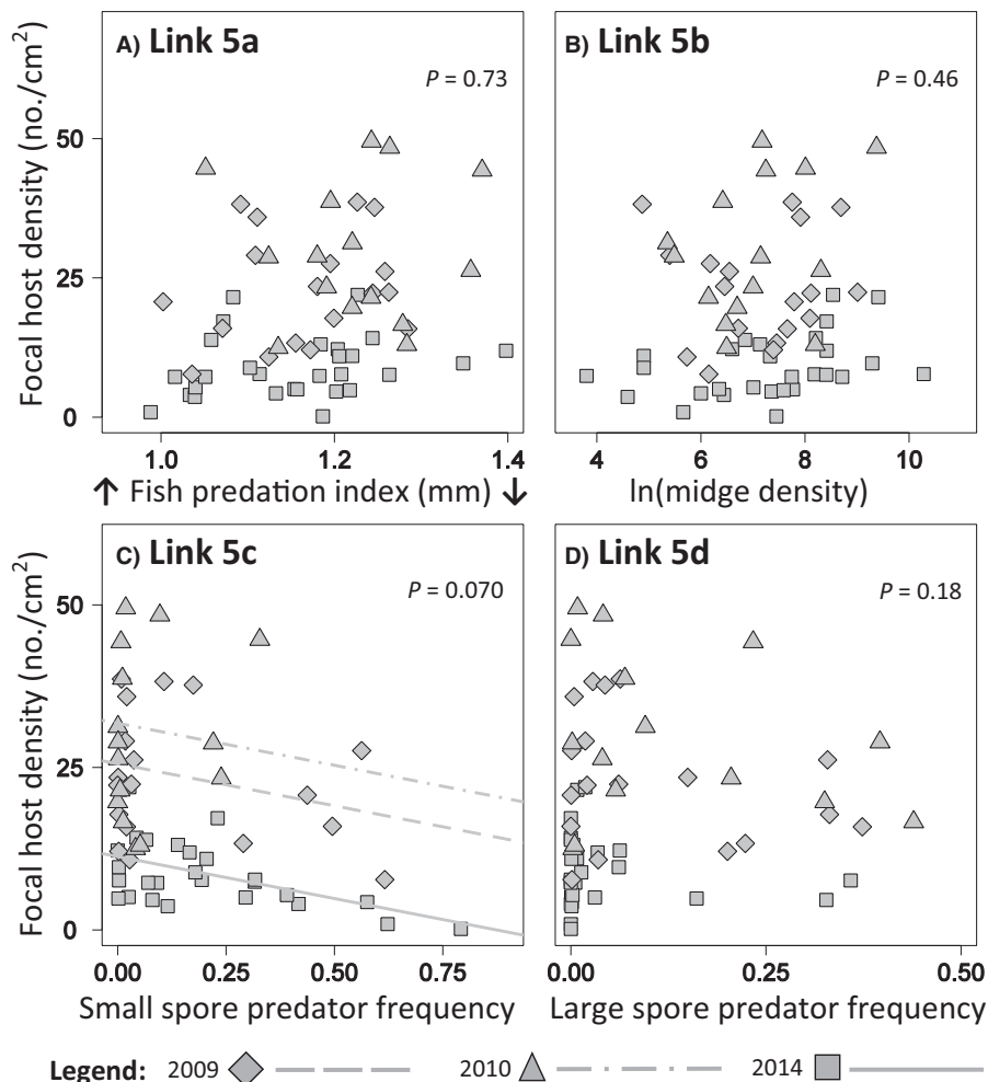
FIG. 4. Focal host density ( Daphnia dentifera ) was only marginally regulated by small spore predators (Link 5, see Table 2). Each point is a lake population in a given year. Focal host density was not reduced by (A) fish predation intensity or (B) midge predator density (measured as no./m 2 ; both are predators of focal hosts). (C) Focal host density was marginally lower in lakes with higher frequencies of small spore predators ( Ceriodaphnia ), but (D) not in lakes with higher frequencies of large spore predators ( D. pulicaria ; both spore predators compete with focal hosts). Regression models were fit with random “lake” effects, fixed “year” effects, and flexible variance functions to account for heteroscedasticity in the data.
