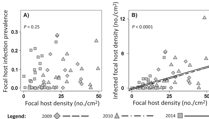
FIG. 1. Overall density of focal hosts ( Daphnia dentifera ) (A) does not drive infection prevalence, but (B) does drive density of infected focal hosts. Each point is a lake population in a given year (2009, 2010, and 2014). Infection prevalence is mean proportion of focal hosts infected during an epidemic season. Infected host density is mean density of infected focal hosts over the same time period. Regression models were fit with random “lake” effects, fixed “year” effects, and flexible variance functions to account for heteroscedasticity in the data.
