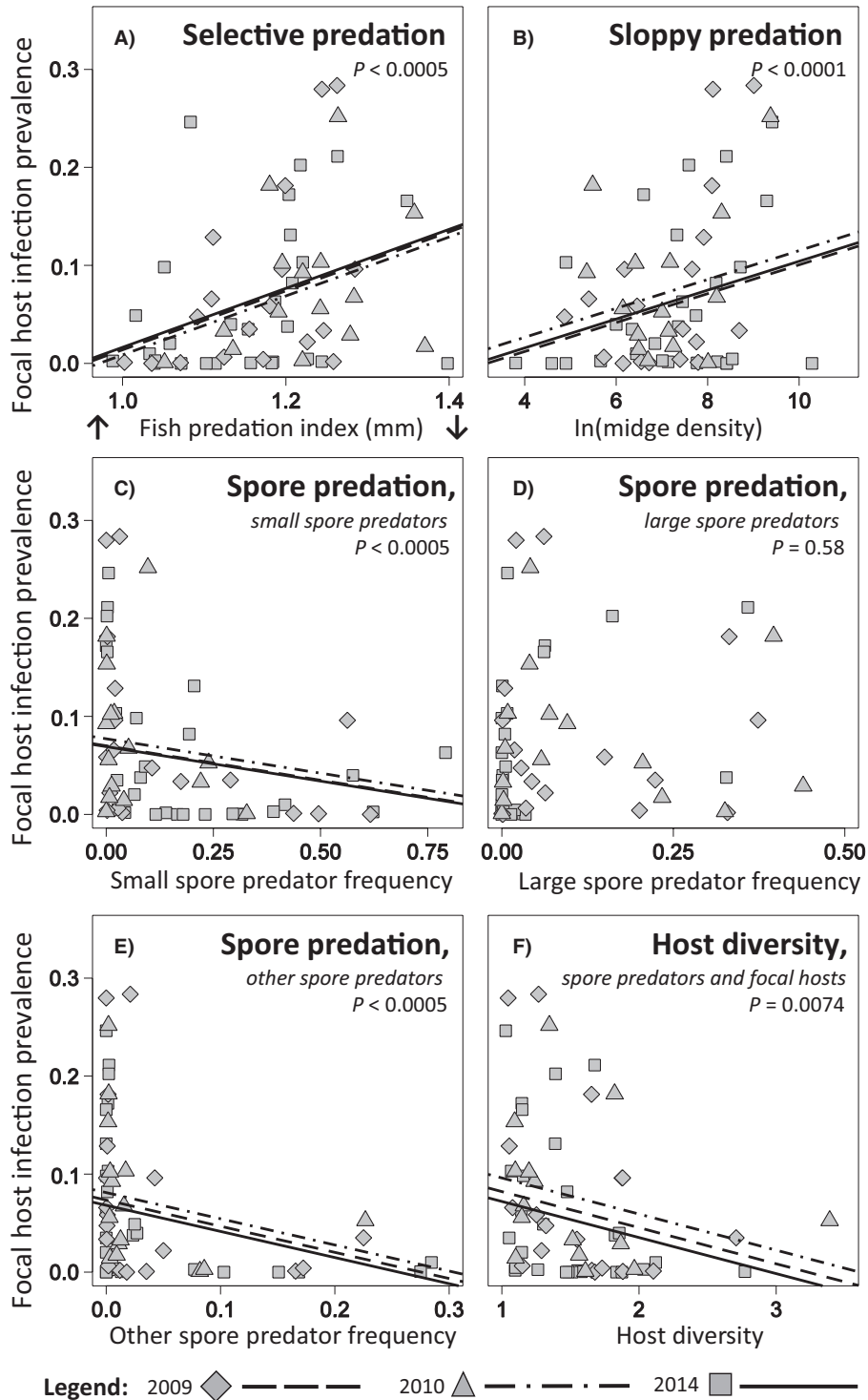
FIG. 2. Three modes of predation (Table 1) correlate with infection prevalence of the focal host zooplankton ( Daphnia dentifera ). Infection prevalence is mean proportion of focal hosts infected during an epidemic season. Each point is a lake population in a given year. (A) Selective predation: fish predation is indexed by body size of adult focal hosts (mm). Smaller size means more fish predation ( \uparrow ); larger size means less ( \downarrow ). More selective fish predation (left on x-axis) is correlated with lower infection prevalence. (B) Sloppy predation: more sloppy midge predators ( Chaoborus ; density measured as no./m 2 ) are correlated with higher infection prevalence. (C–E) Spore predation: (C) high frequencies within the host community of small spore predators ( Ceriodaphnia ) correlated with lower infection prevalence. (D) Frequency of large spore predators ( D. pulicaria ) did not, but (E) frequency of other spore predators did. (F) Host diversity: finally, higher host diversity (measured as the inverse of Simpson's diversity index, including focal hosts and spore predators) also correlated with lower infection prevalence, consistent with a dilution effect. Regression models were fit with random "lake" effects, fixed "year" effects, and flexible variance functions to account for heteroscedasticity in the data.
