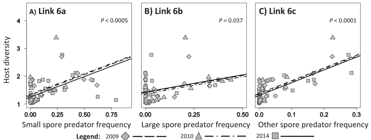
FIG. 5. Diversity of the host community (i.e., focal hosts [ Daphnia dentifera ] and spore predators; measured as the inverse of Simpson's diversity index) was strongly regulated by frequency of each group of spore predators. Spore predators are themselves hosts, but are all rarer than focal hosts. Each point is a lake population in a given year. Higher frequencies of (A) small spore predators ( Ceriodaphnia ), (B) large spore predators ( D. pulicaria ), and (C) other spore predators all increased host diversity. Regression models were fit with random "lake" effects, fixed "year" effects, and flexible variance functions to account for heteroscedasticity in the data.
