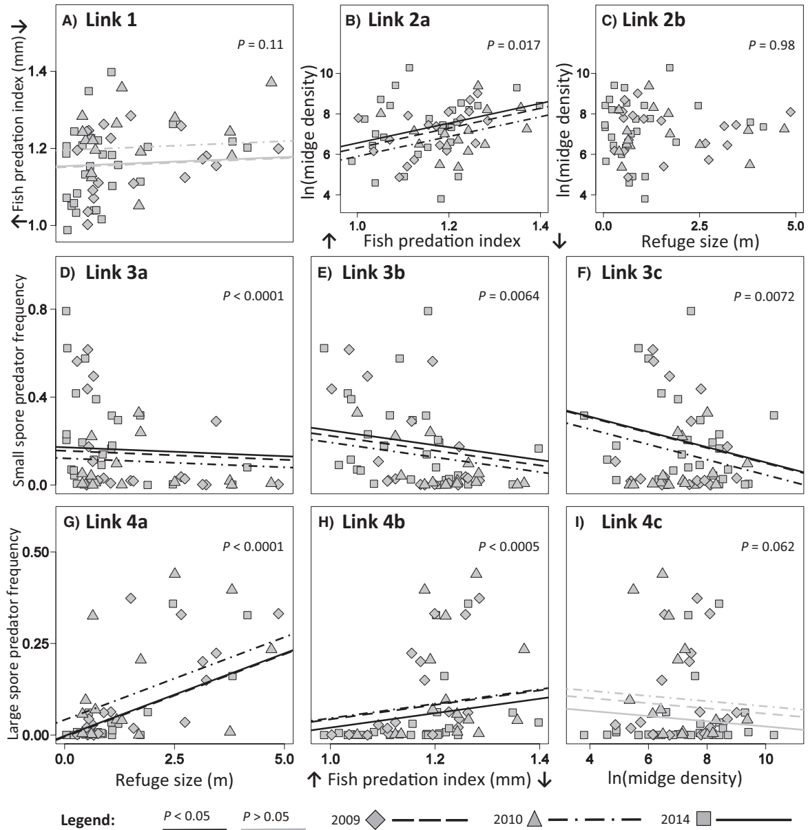
FIG. 3. Predators were regulated by habitat structure and trophic interactions with other predators (Links 1–4; see Table 2). Each point is a lake population in a given year. (A) Small refuge habitats had only marginally more fish predation. (B) More intense fish predation (smaller adult focal host size; left on x-axis) correlated with fewer sloppy midge predators ( Chaoborus ; density measured as no./m 2 ). However, (C) refuge size did not predict midge density. Small spore predators were more frequent when (D) refuge size was smaller, (E) fish predation intensity was higher, and (F) midge density was lower. In contrast, large spore predators were more frequent when (G) refuge size was larger, (H) fish predation intensity was lower, and (I) midge density was lower (marginally). Regression models were fit with random “lake” effects, fixed “year” effects, and flexible variance functions to account for heteroscedasticity in the data.
